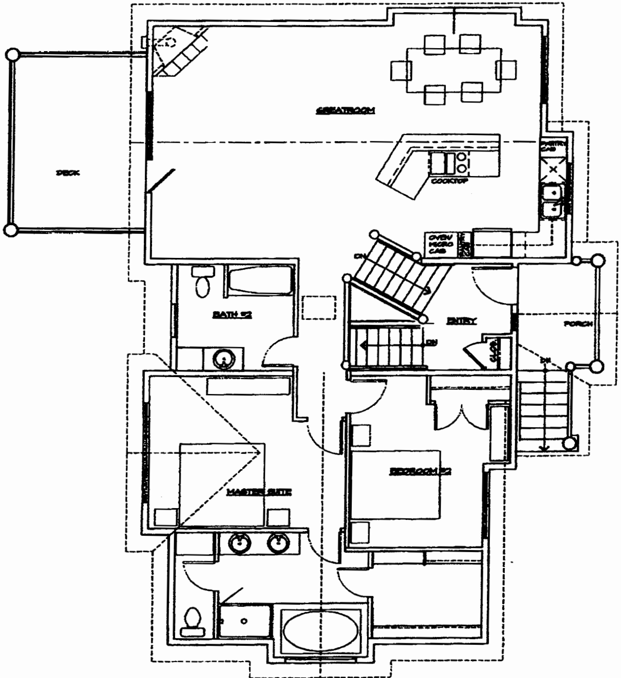
410 KESTREL LANE UPPER FLOOR PLAN
